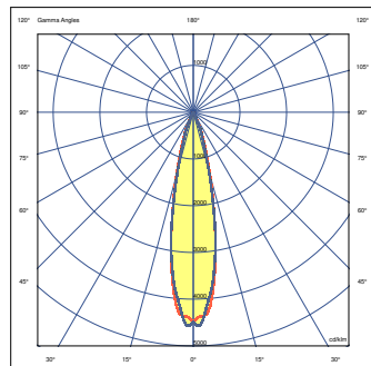
40 DEGREE 5000K 70CRI
