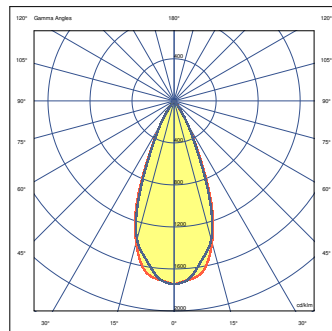
60 DEGREE 5000K 70CRI
