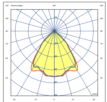
110 DEGREE 5000K 70CRI
