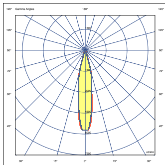
25 DEGREE 5000K 70CRI
